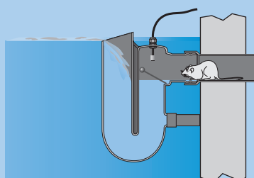
Disposal of the floating layer
